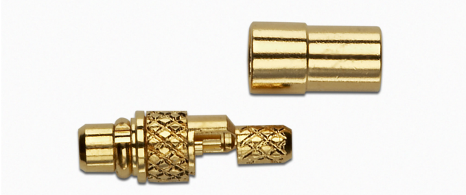
Model 73024 MMCX PLUG STRAIGHT CRIMP, RG178
